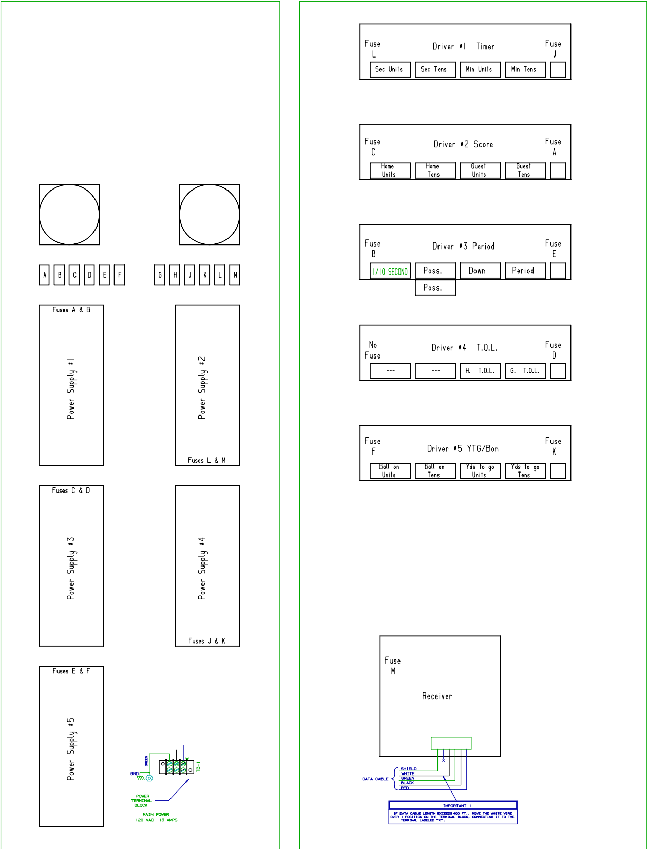
CONTROLLER ASSEMBLY
